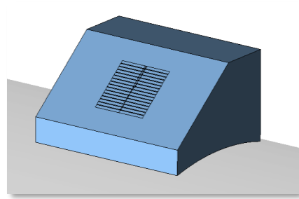
Wedges are contoured along the probe primary axis
